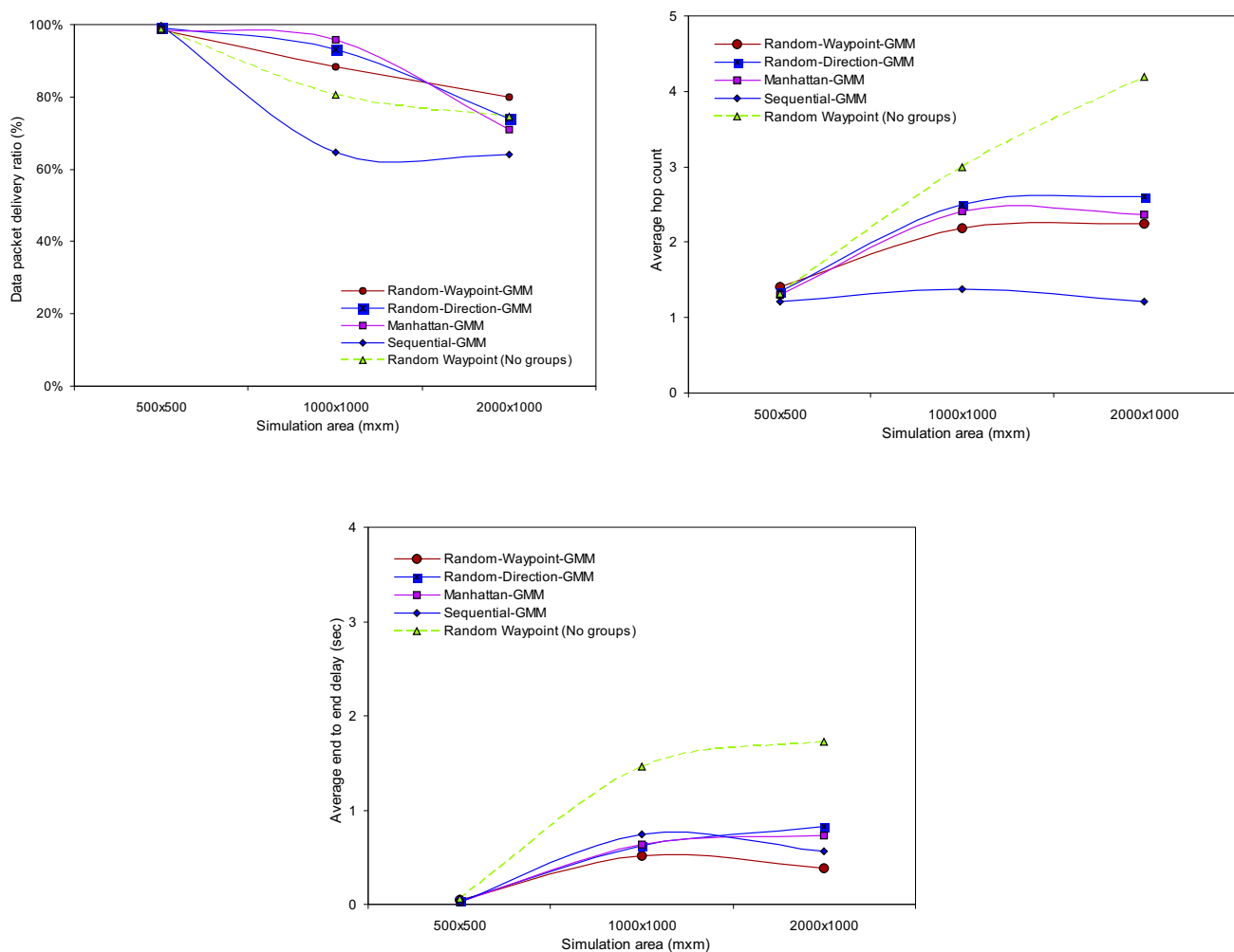
Fig. 7. Performance results for the 100 nodes MANET with five different mobility models as a function of the simulation area size
