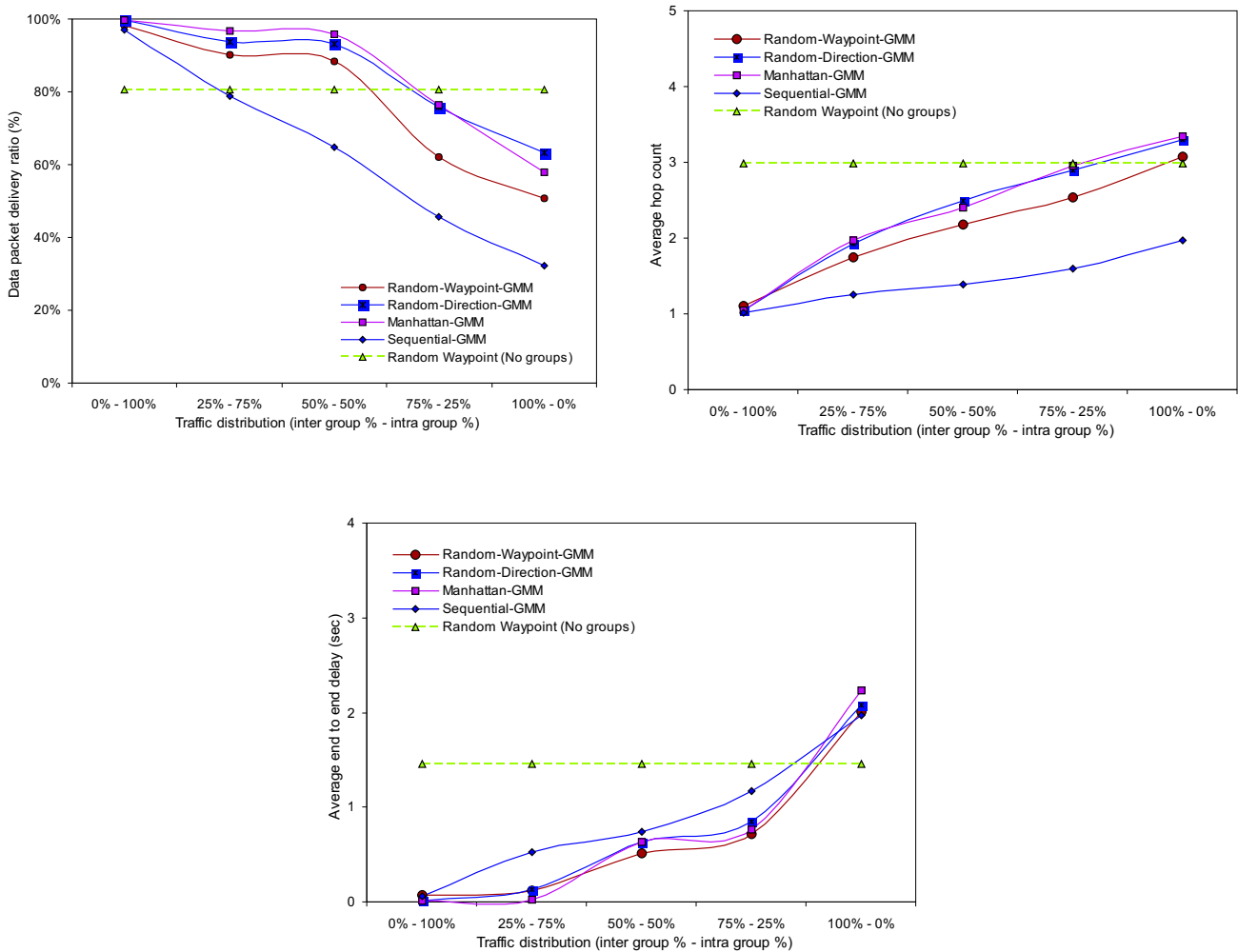
Fig. 4. Performance results for the 100 nodes MANET with five different mobility models as a function of traffic distribution
