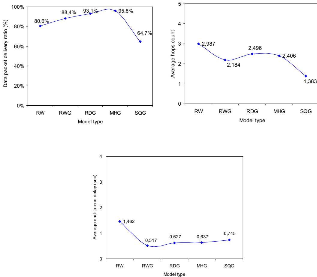
Fig. 3. Performance results for the 100 node MANET basic scenario using the different mobility models.
