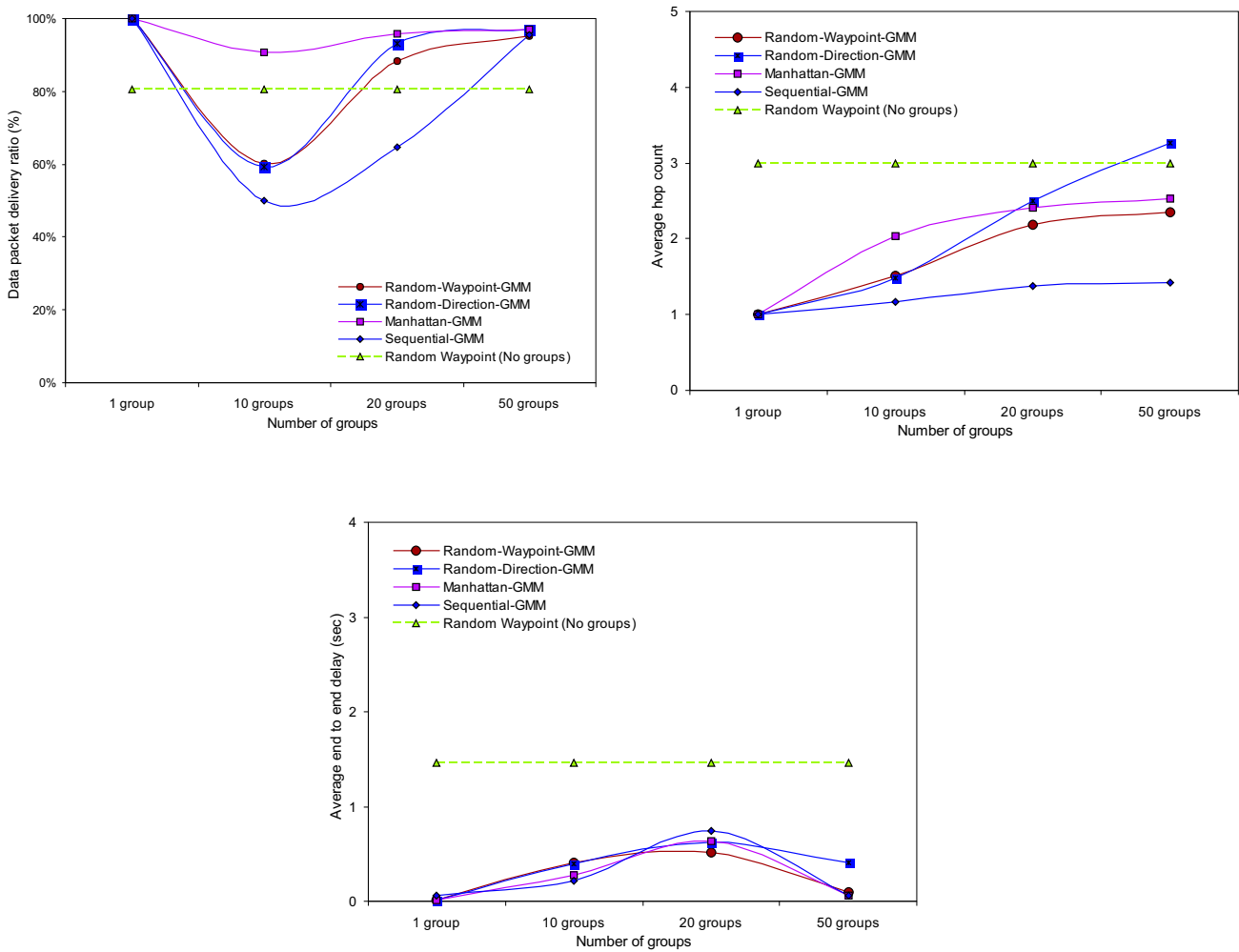
Fig. 6. Performance results for the 100 nodes MANET with five different mobility models as a function of the number of groups
