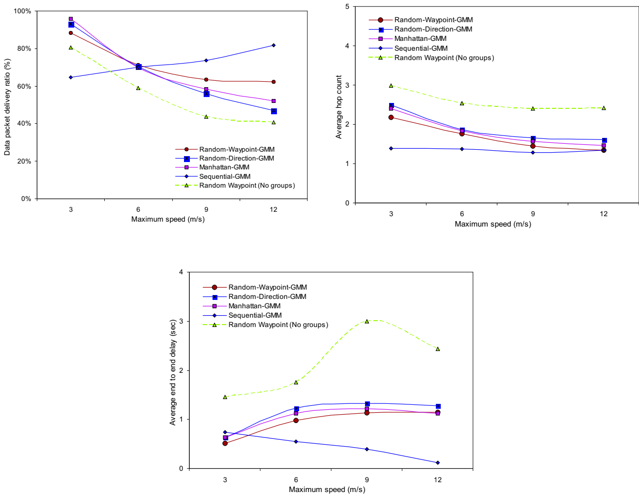
Fig. 5. Performance results for the 100 nodes MANET with five different mobility models as a function of the maximum node speed
